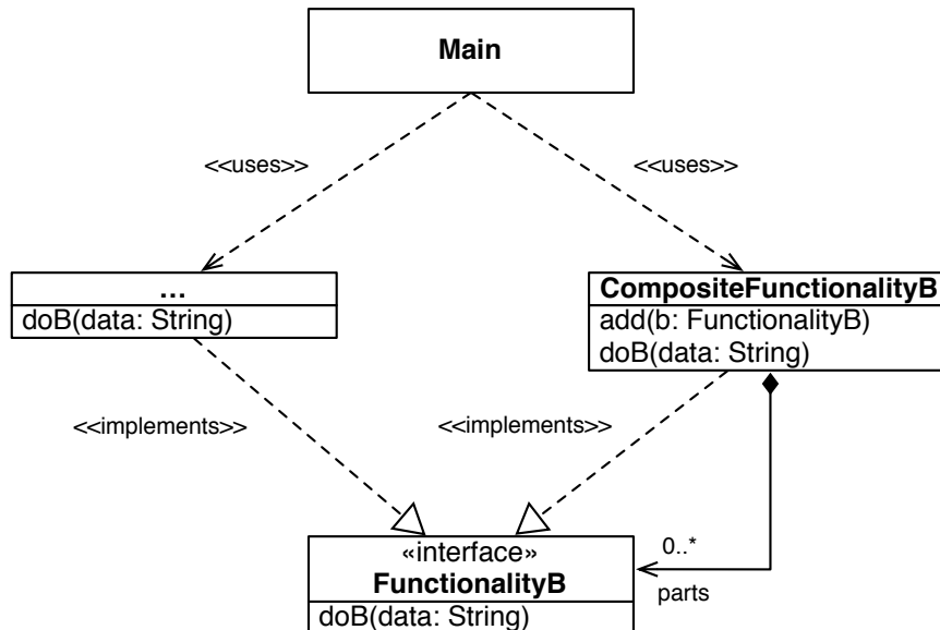
Figure 4: UML class diagram for a composite callback
