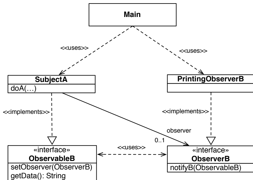
Figure 6: UML class diagram for observers that pull
