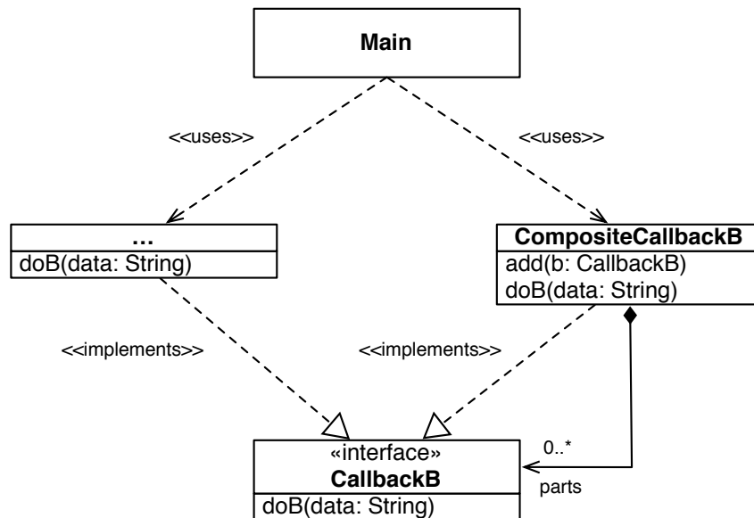
Figure 4: UML class diagram for a composite callback
